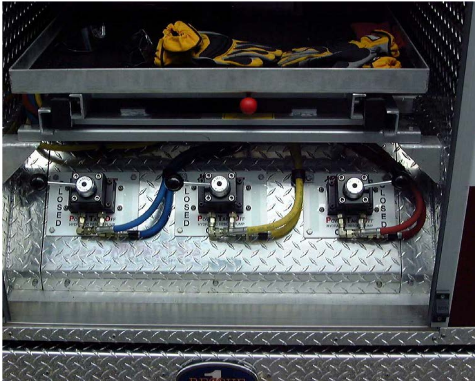
Three tool - Rear Compartment Installation
